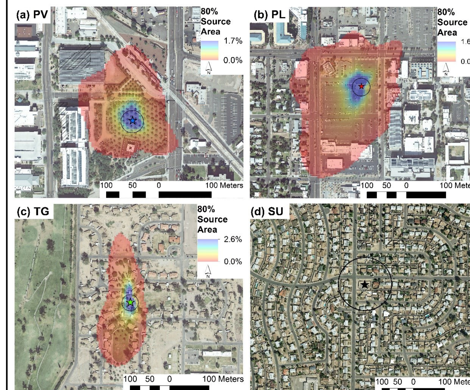
Fig. 2 Study site orthoimagery with the 80% source areas (colored 5 m pixels with percent contribution) and radiometer footprints (black circles) at: (a) PV, (b) PL, (c) TG and (d) SU sites.
