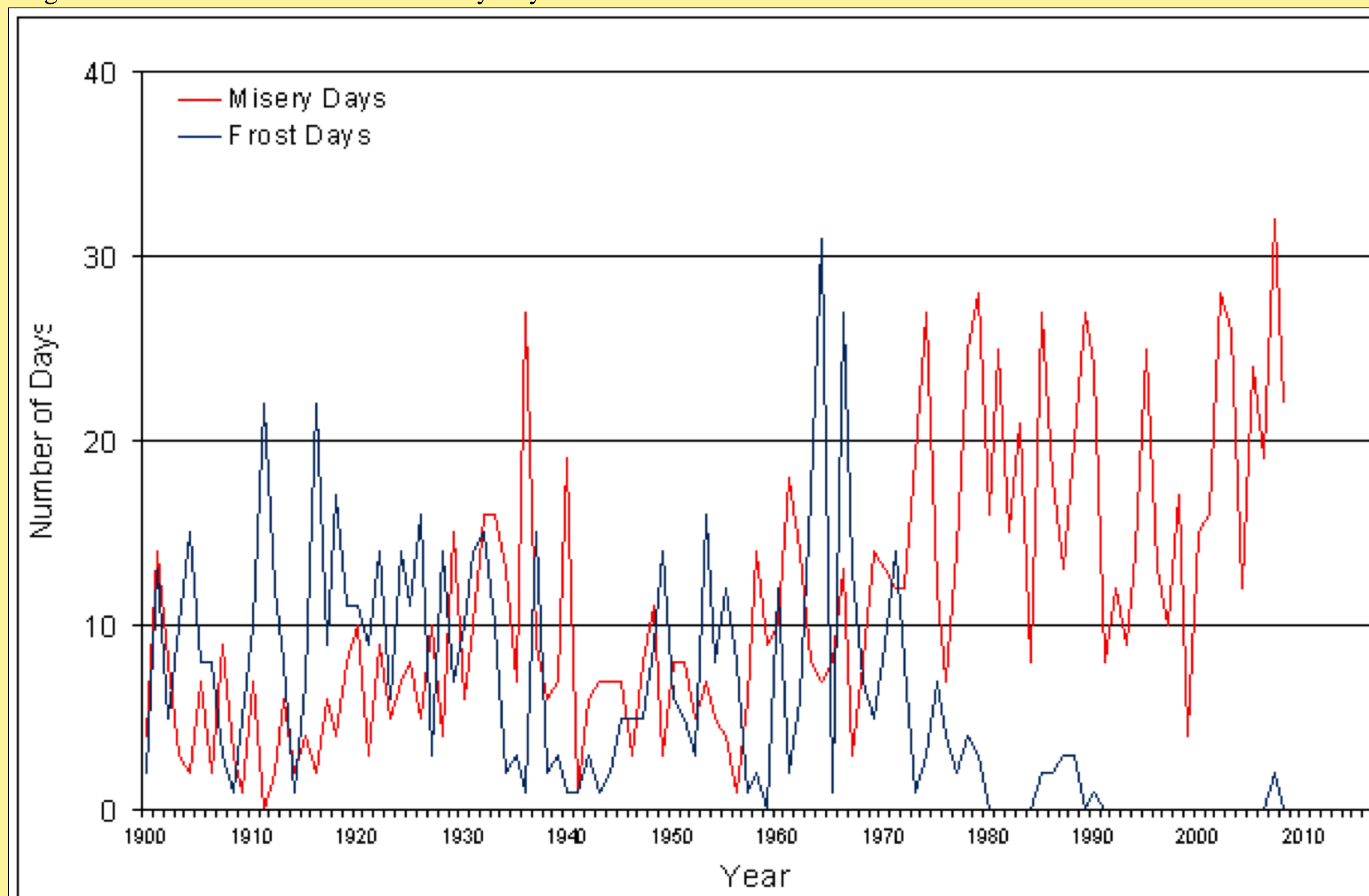
Figure 3: Occurrences of Frost and Misery Days from 1896-2009
