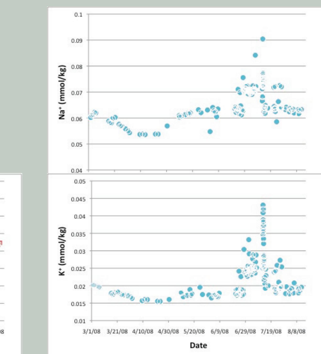
Figures 6 & 7. Concentrations of sodium (top) and potassium through time.
