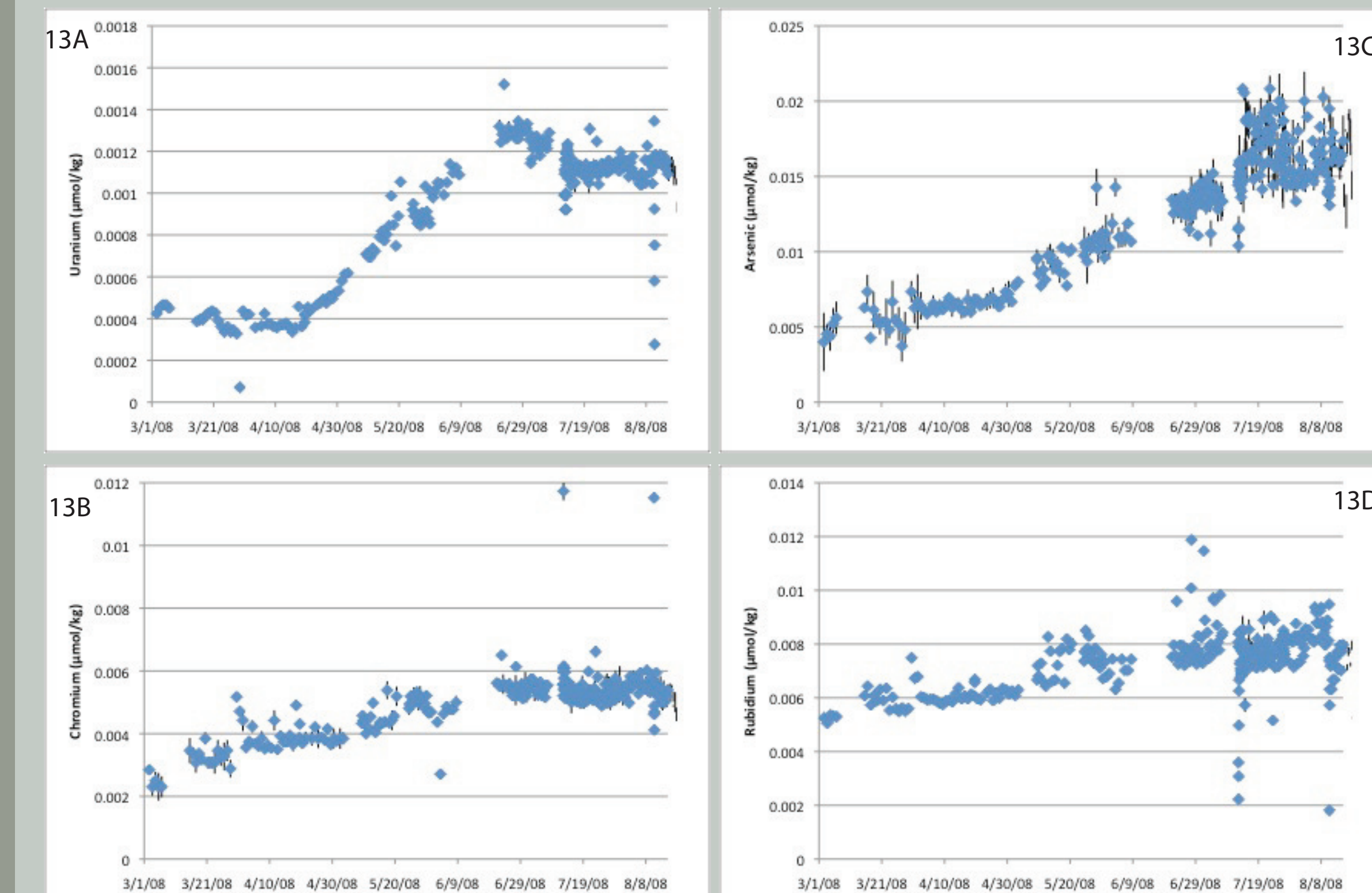
Figure 13. Concentrations of uranium, chromium, arsenic and rubidium (13A, B, C and D, respectively) through time. All four elements show similar seasonal concentration trends, with an increase to a summer plateau.
