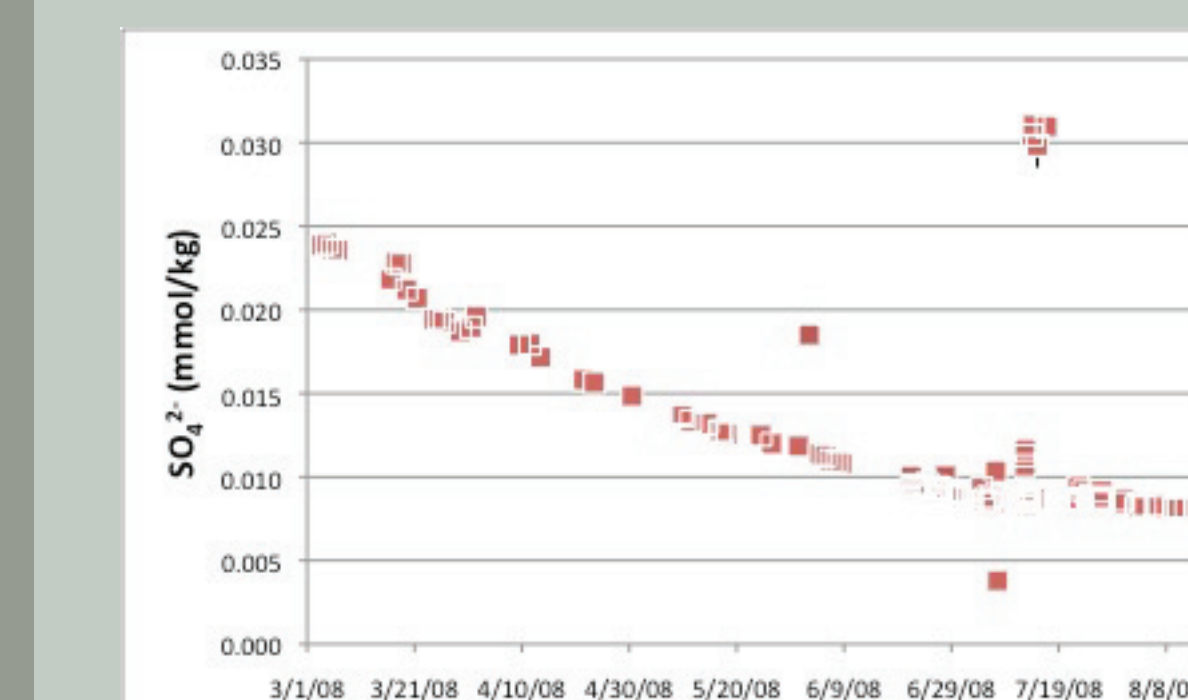
Figure 11. Concentration of sulfate through time.
