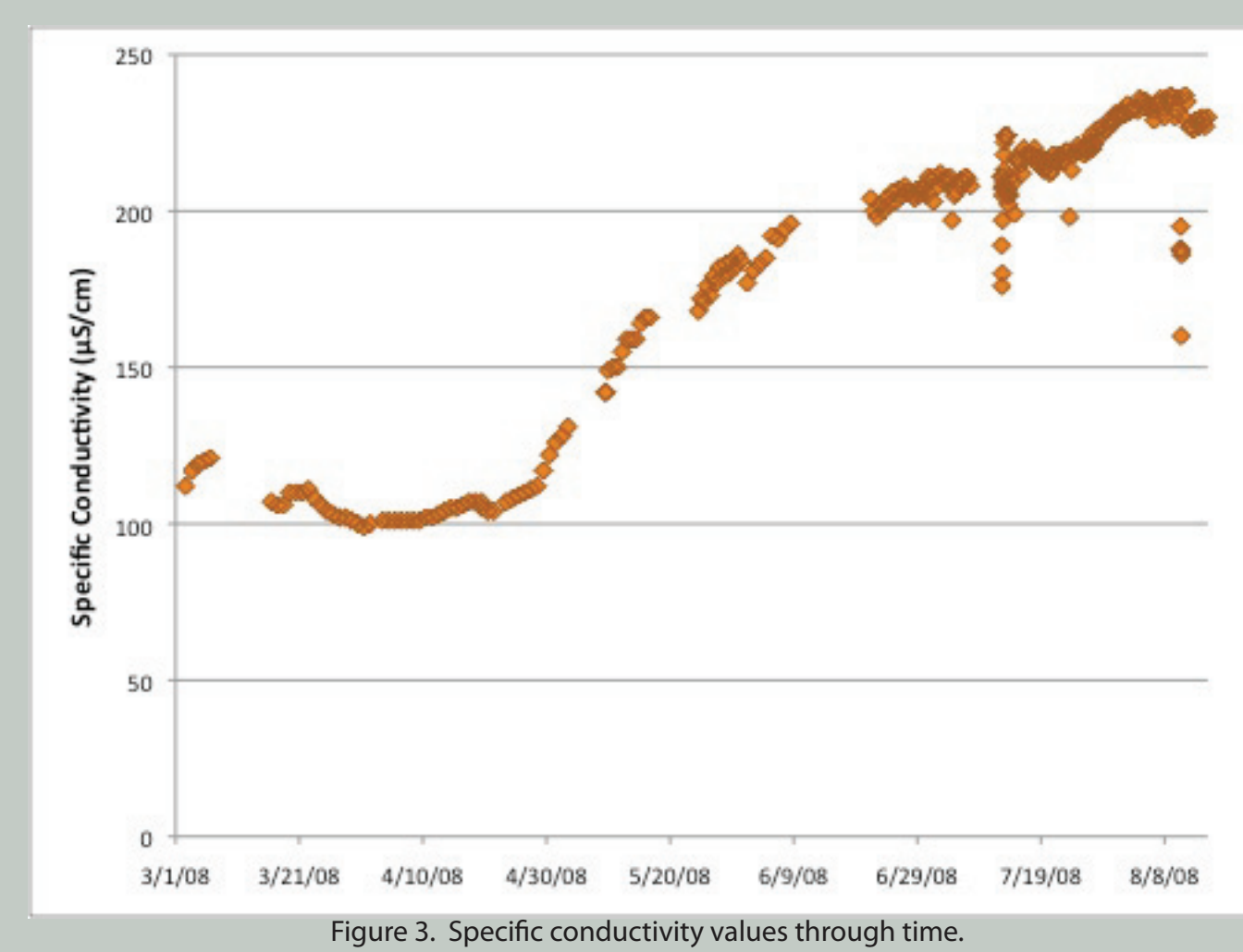
Figure 3. Specific conductivity values through time.
