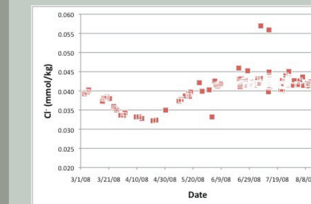
Figure 8. Concentration of chloride through time.
