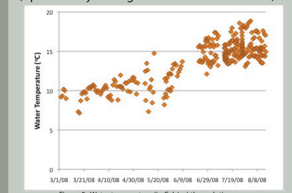
Figure 5. Water temperature (in Celsius) through time.
